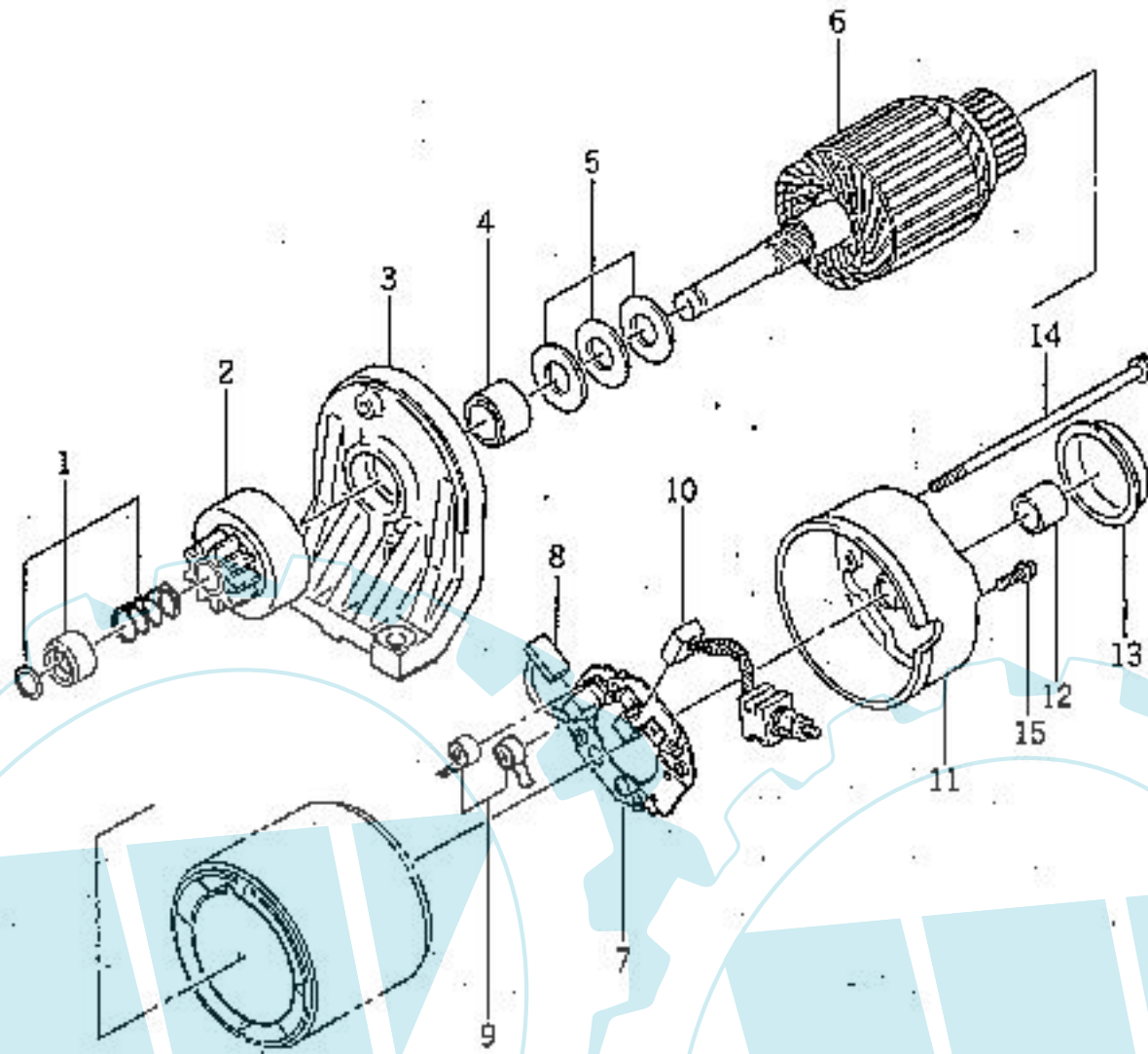
Fig. S-1 ELECTRIC STARTER
