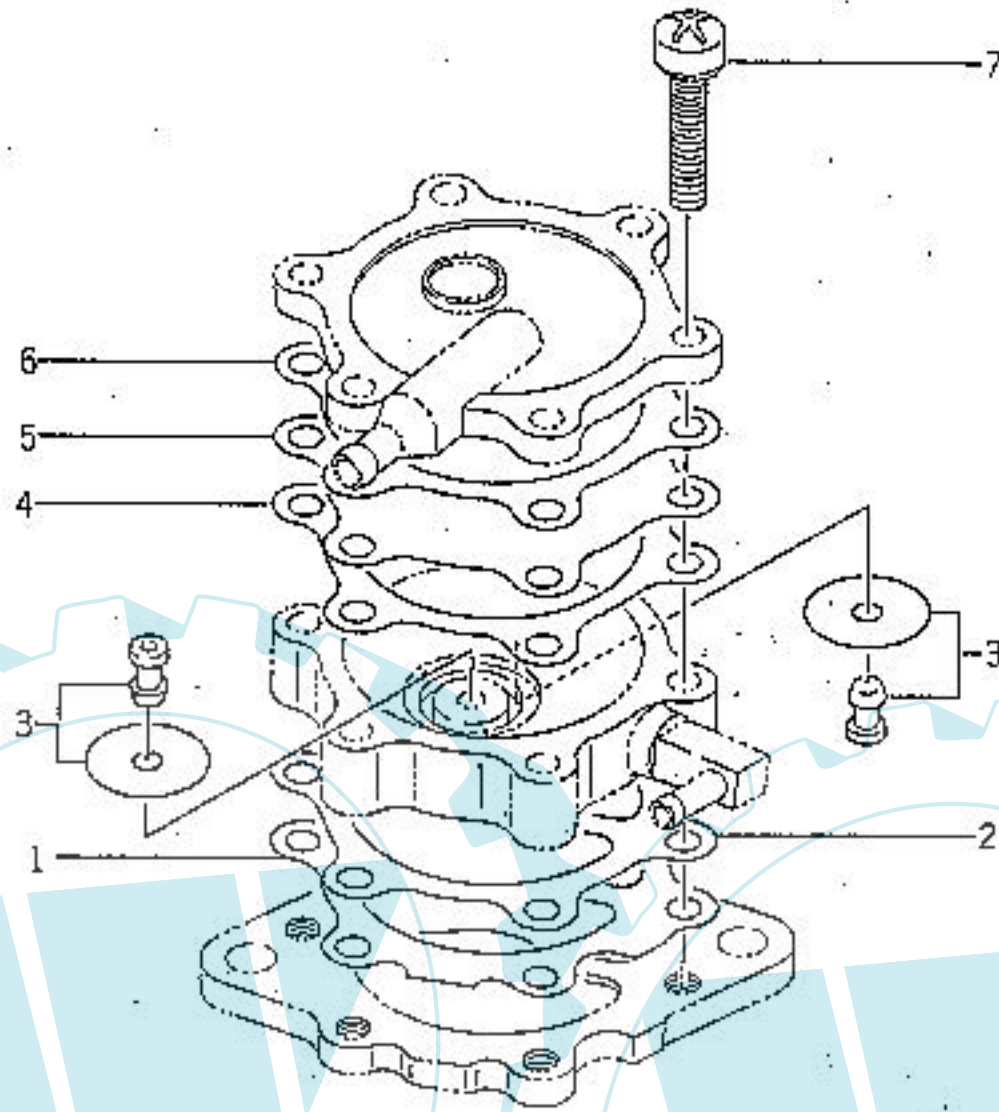
Fig. P-1 FUEL PUMP
