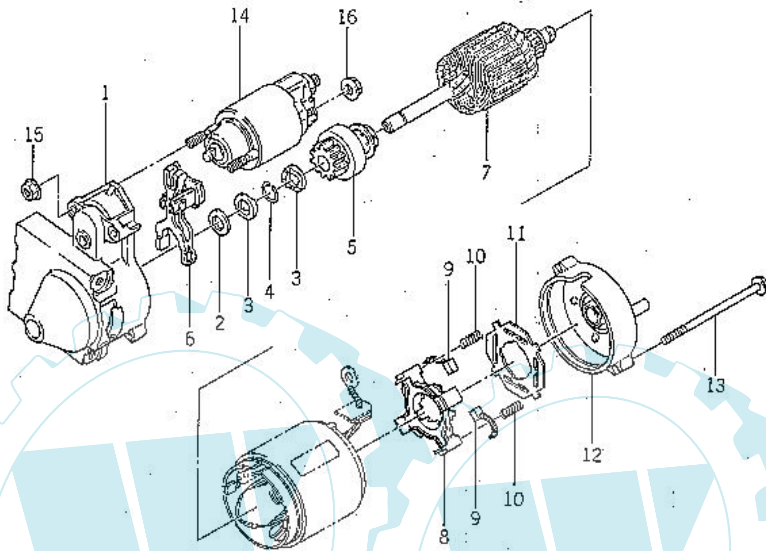
Fig.S-2 ELECTRIC STARTER
