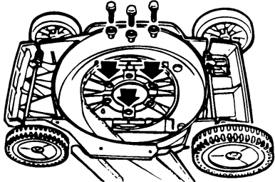
MOTOR MOUNT (Bottom View): Items 28, 29 assembled in 3 locations indicated.
