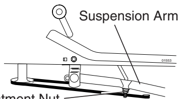
Lift Link Adjustment Nut
